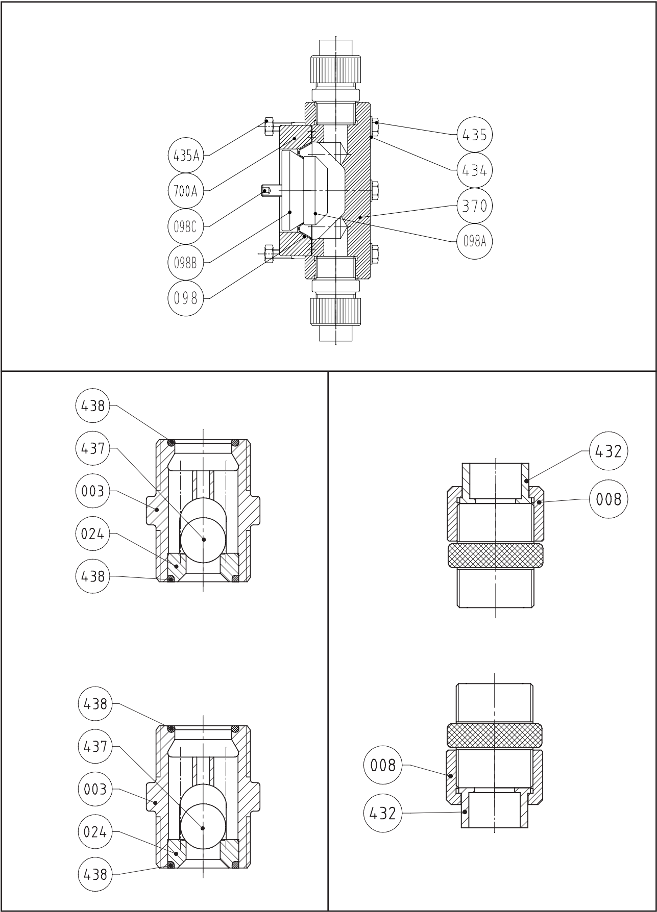
图5-14 GM0090~GM0500 PVC, PVDF & 混合物液力端
